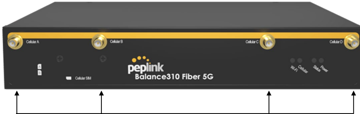
Cellular (MIMO 4 x SMA)
