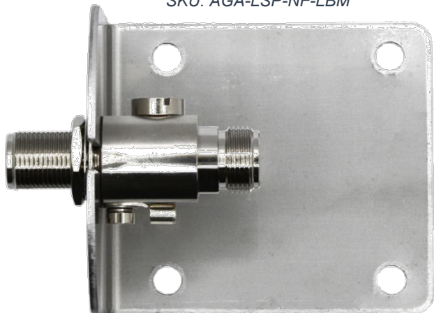
Surge Protector w/ L-Bracket Mount Kit SKU: AGA-LSP-NF-LBM
